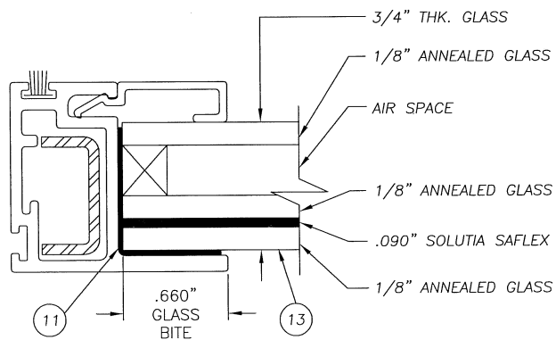
GLAZING DETAIL
