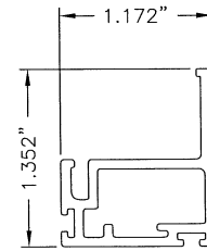
5 SASH STILE VEKA #SH45
