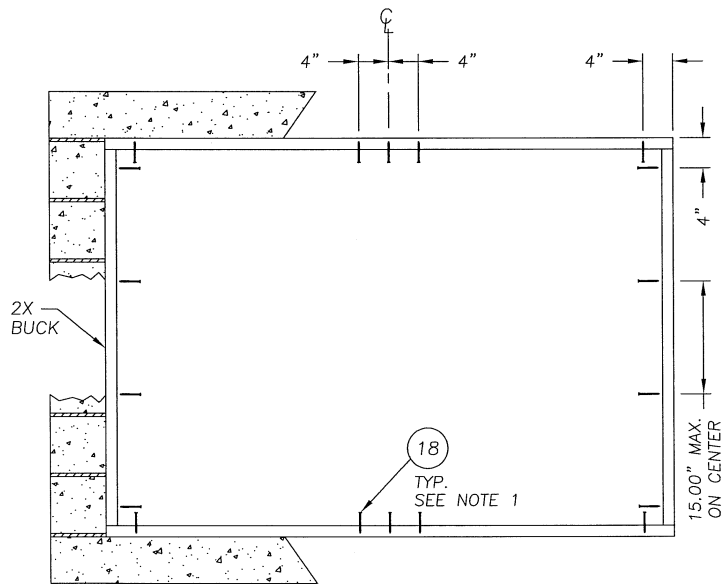
BUCK ANCHORING
