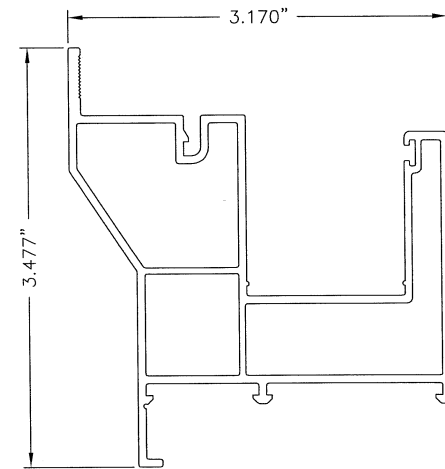
1 MASTER FRAME VEKA #PI3101
