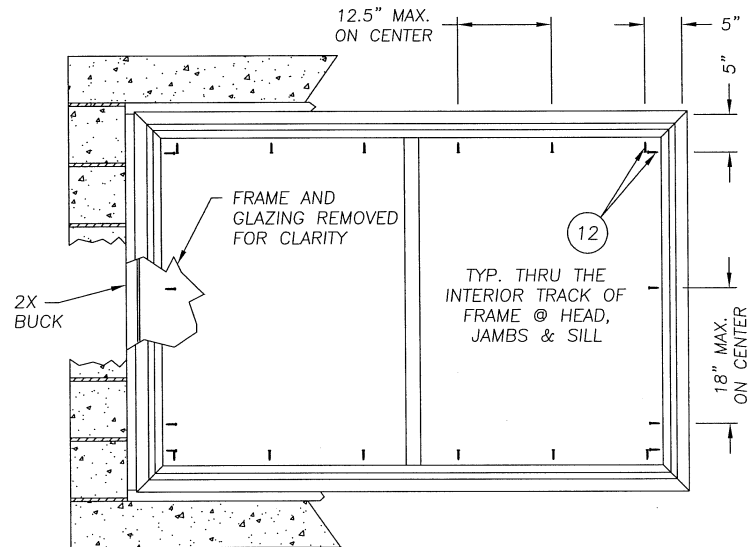
FRAME ANCHORING
