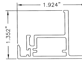
4 LOCK RAIL VEKA #SH46
