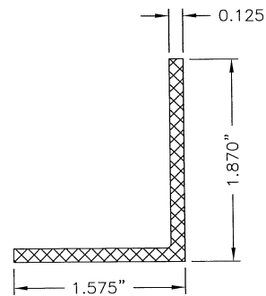
7 FRAME REINFORCEMENT VEKA #RFSSA2101 AOM
