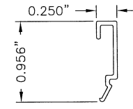
6 GLAZING BEAD VEKA #BV75
