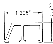
3 SILL TRACK VEKA #DS3008
