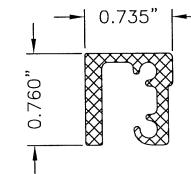
8 MULLION REINFORCEMENT VEKA #RFSH34 AOM
